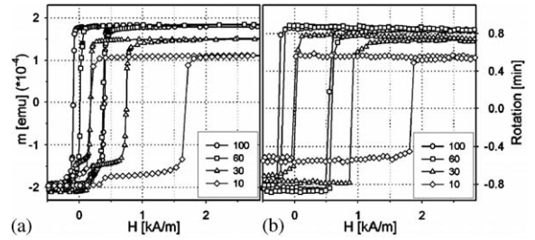
Fig. 3. Minor hysteresis loops of MTJ; change of field step every 5 s—R-VSM (a) and 5 ms—MOKE (b).
