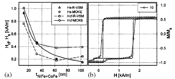
Fig. 4. (a) Free layer thickness dependence of H_s and H_{cf} measured by R-VSM and MOKE; the solid line fitted for J = 1.04 \times 10^{-5} \text{ J/m}^2 (b) Calculated (solid line) and measured by R-VSM (circles) minor loops of free layer.
